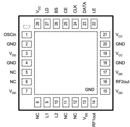
28-Pin 5x5 LLP (LQ) Package
