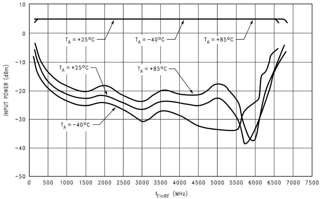
LMX2434 FinRF Input Power Vs Frequency V CC = EN = 2.35V
