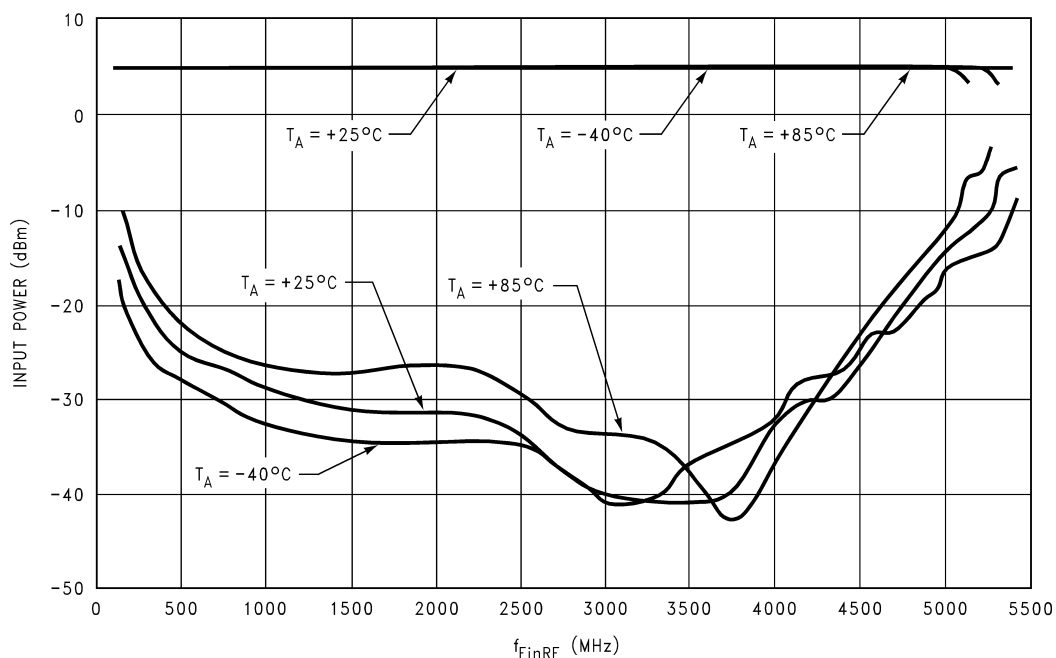
LMX2433 FinRF Input Power Vs Frequency V CC = EN = 2.75V
