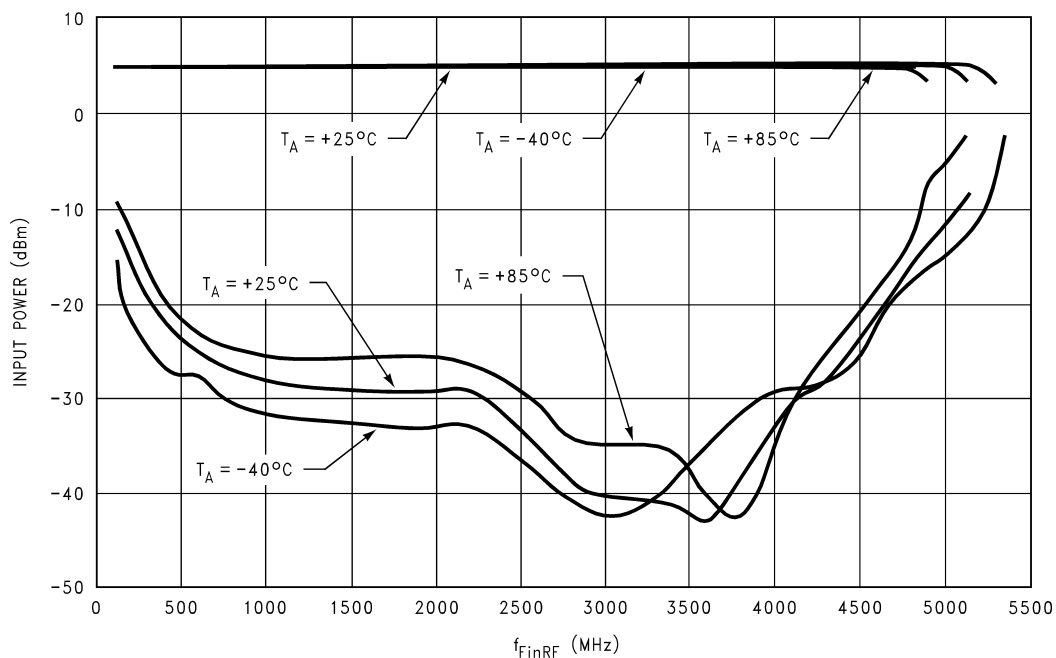
LMX2433 FinRF Input Power Vs Frequency V CC = EN = 2.25V
