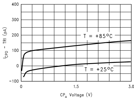
I CPO TRI-STATE vs CP O Voltage
