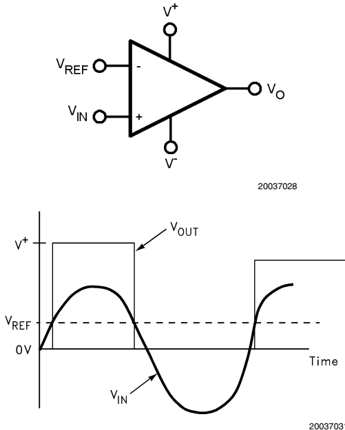
FIGURE 1. Basic Comparator
