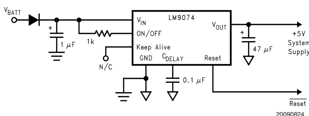
FIGURE 2. Control Logic Not Used
