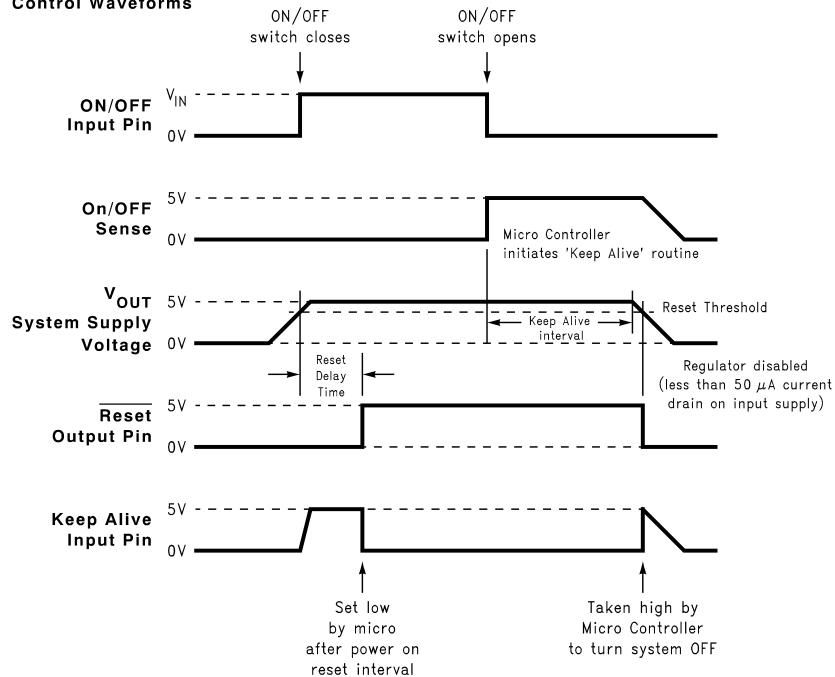
Control Waveforms
