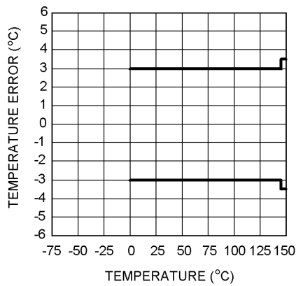
Temperature Error
