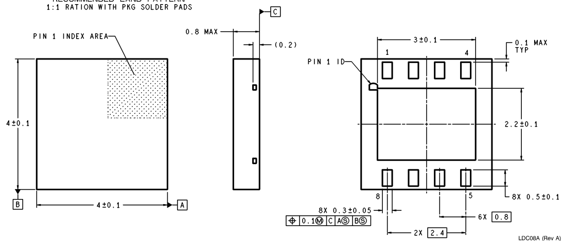
8-Pin LLP NS Package Number LDC08A
