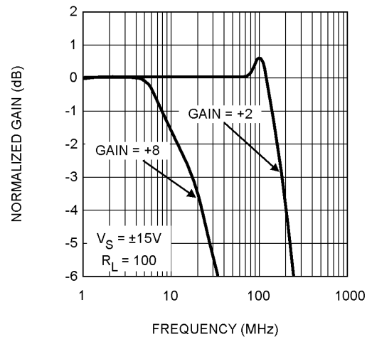
Frequency Response
