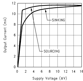
Short Circuit Current vs Supply Voltage
