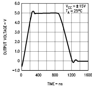
Unity Gain Large Signal Pulse Response
