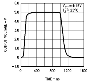
Large Signal Pulse Response for Gain 10
