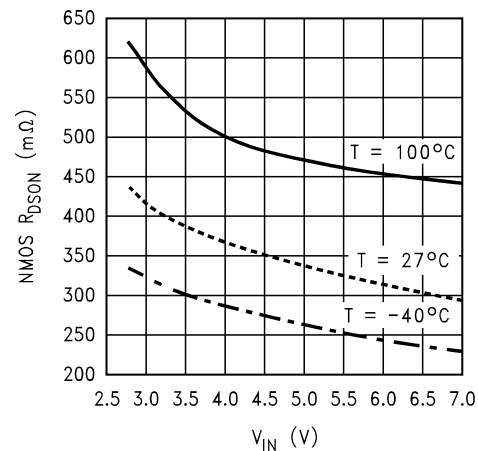
NMOS R_{DS(on)} vs. V_{IN} ( I_{SW} = 300 mA)
