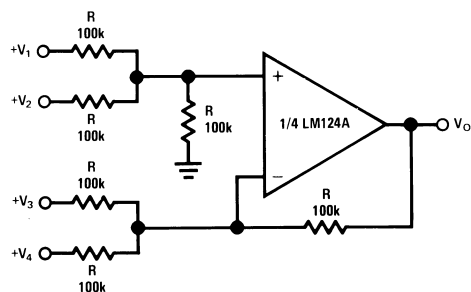
DC Summing Amplifier ( V_{\text{IN}}\text{'S} \geq 0\text{ V}_{\text{DC}} and V_{\text{O}} \geq V_{\text{DC}} )
