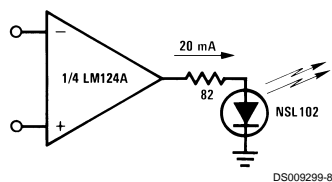
LED Driver
