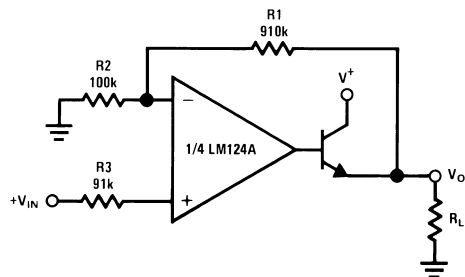
Power Amplifier
