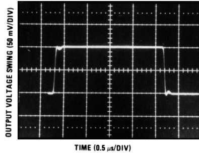
LF156 Small Signal Pulse Response, A_V = +1
