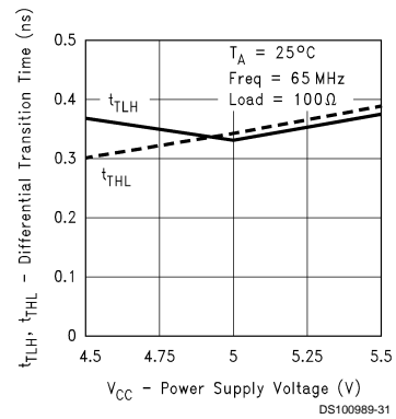
Differential Transition Time vs Power Supply Voltage
