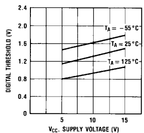
Digital Input Threshold vs. V CC
