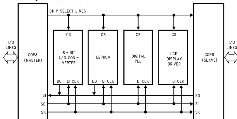
FIGURE 8. MICROWIRE/PLUS Application
