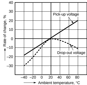
8-(2). Rate of change in pick-up and drop-out voltage (2C) RG2-12V 5 pcs.
