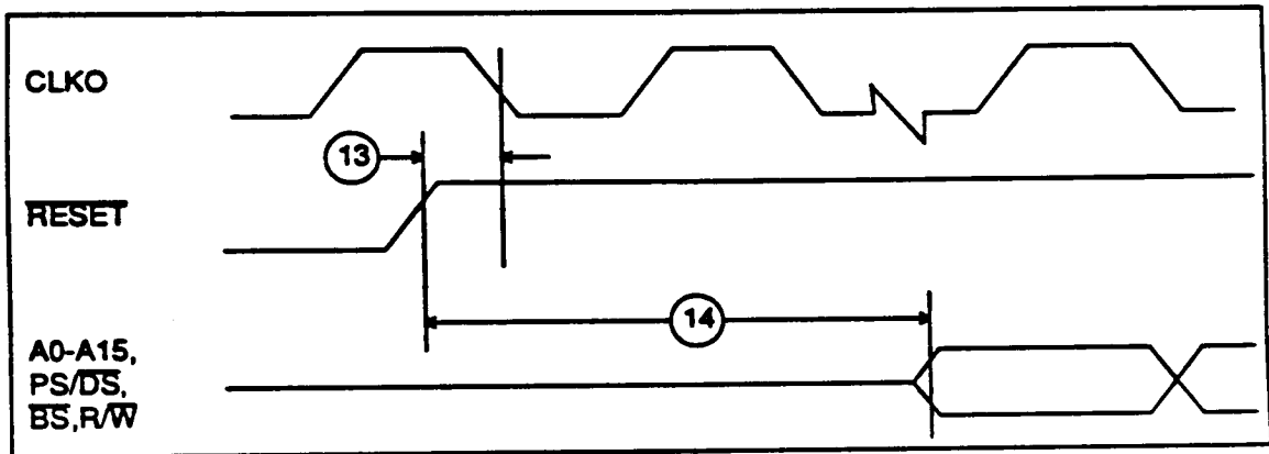
Interrupt Figure 2. Synchronous Reset Timing
