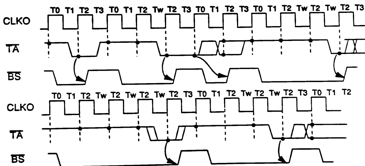
Figure 3 TA Controlled Accesses
