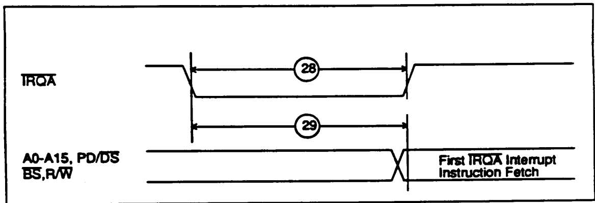
WAIT and STOP Figure 3. Recovery from Stop State Using TRQA Interrupt Service
