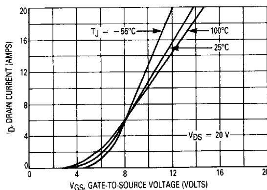
Figure 4. Transfer Characteristics
