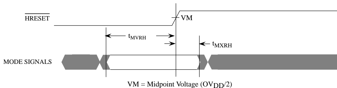
Figure 5. Mode Input Timing Diagram
