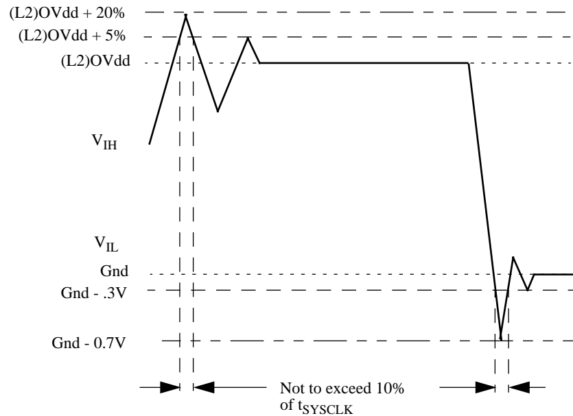
Figure 2. Overshoot/Undershoot Voltage
