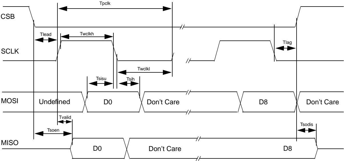
Figure 2. Timing Characteristics
