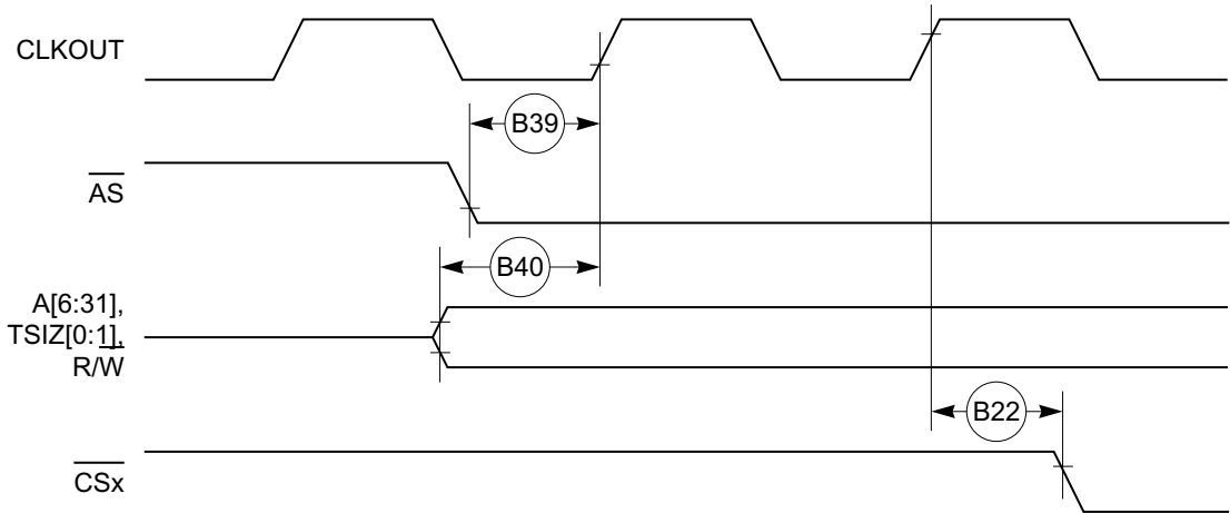
Figure 6-20. Asynchronous External Master Memory Access Timing (GPCM Controlled—ACS = 00)
