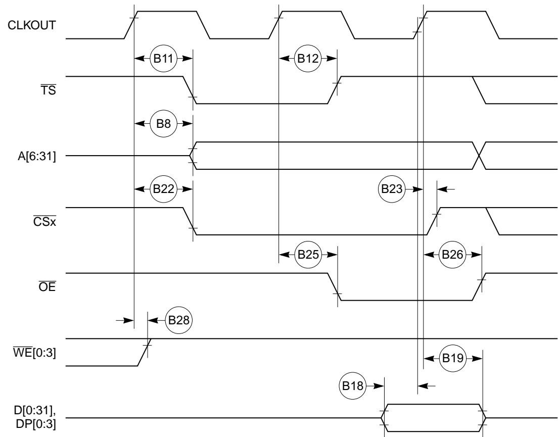
Figure 6-9. External Bus Read Timing (GPCM Controlled—ACS = 00)
