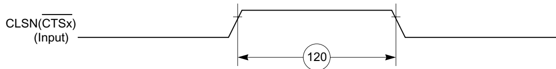
Figure 8-53. Ethernet Collision Timing Diagram
