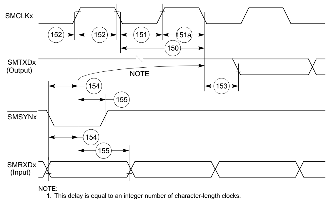
Figure 8-56. SMC Transparent Timing Diagram
