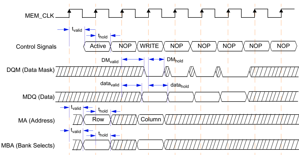
Figure 6 Timing Diagram—Standard SDRAM Memory Write Timing
