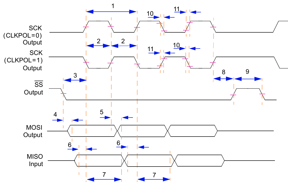
Figure 31 Timing Diagram — SPI Master Mode, Format 0 (CPHA = 0)
