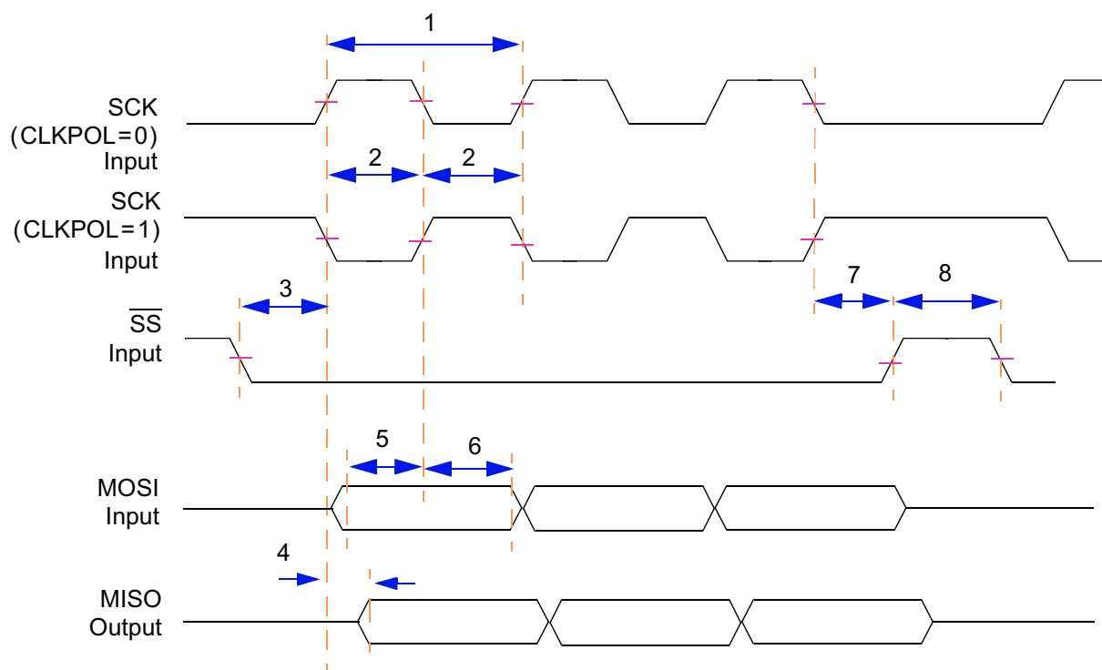
Figure 34 Timing Diagram — SPI Slave Mode, Format 1 (CPHA = 1)
