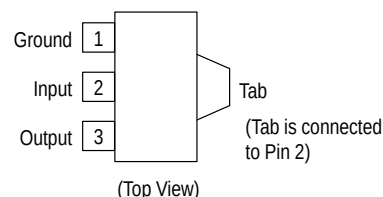
H SUFFIX PLASTIC PACKAGE CASE 1213 (SOT-89)
