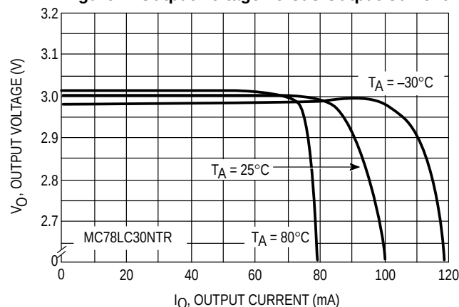
Figure 2. Output Voltage versus Output Current
