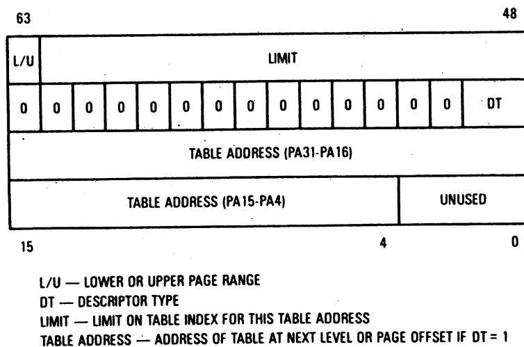
Figure 9-9. Root Pointer Descriptor Format
