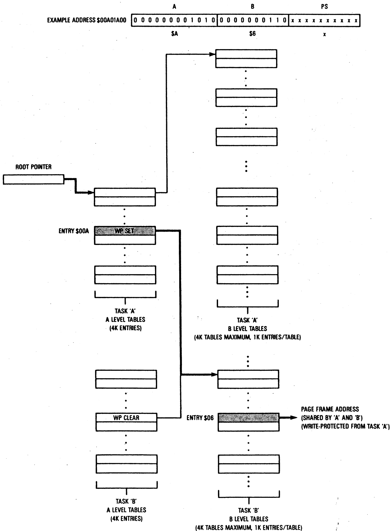
Figure 9-23. Example Translation Tree Using Shared Tables
