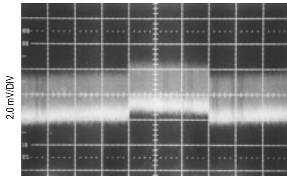
Figure 9. Reference Line Regulation
