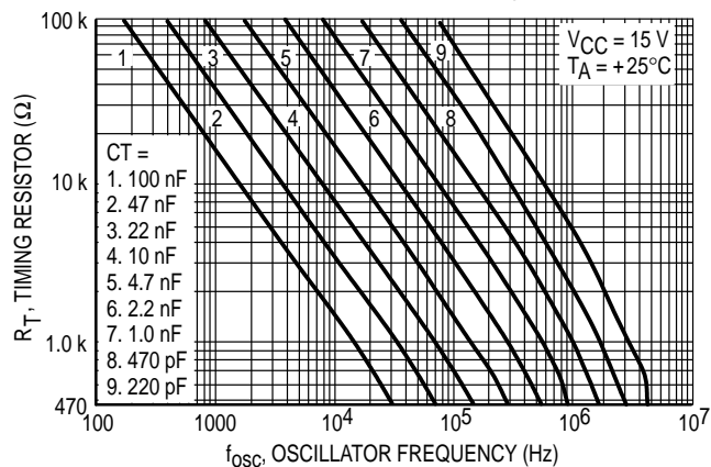
Figure 1. Timing Resistor versus Oscillator Frequency
