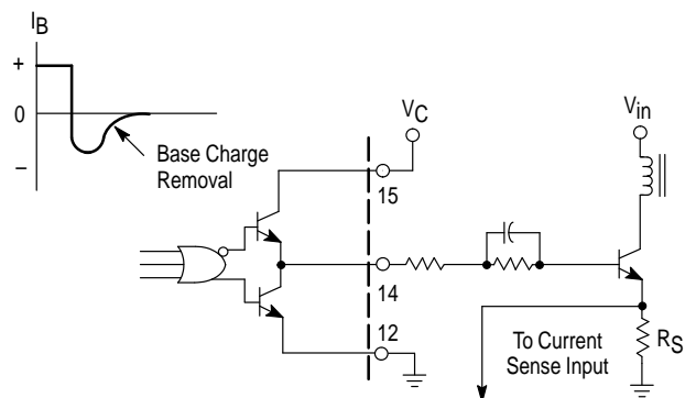
Figure 31. Bipolar Transistor Drive
