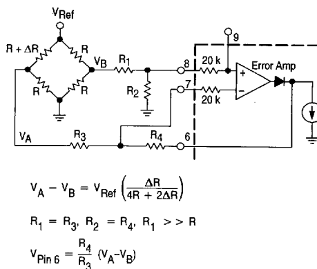
Figure 28. Bridge Amplifier
