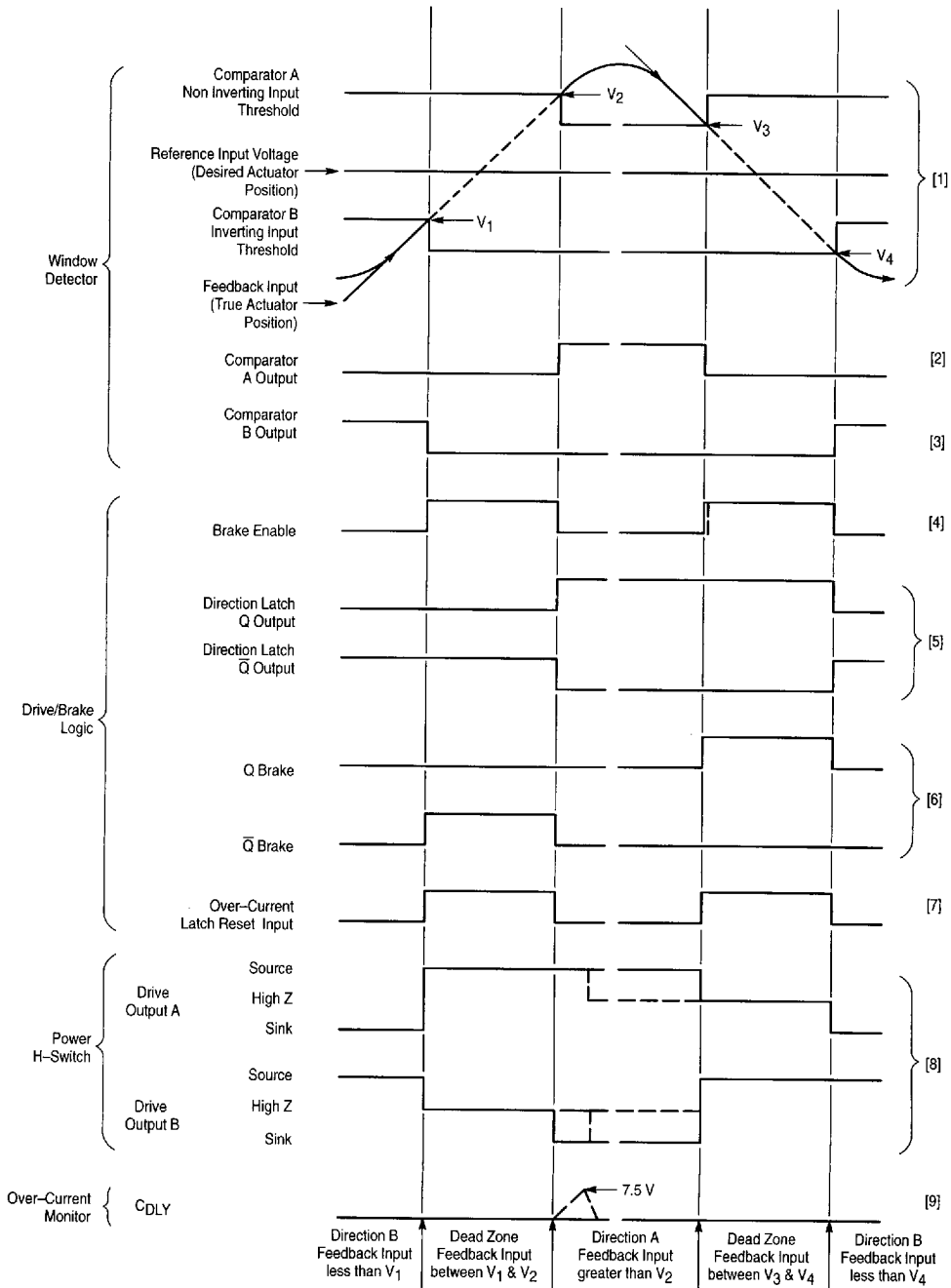
Figure 18. Timing Diagram
