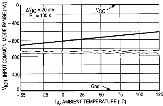
Figure 1. Error Amp Input Common-Mode Voltage Range versus Temperature
