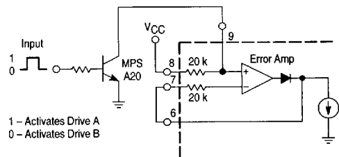
Figure 22. Digital Two Position Servo System
