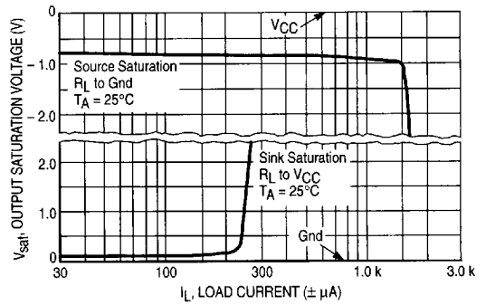
Figure 2. Error Amp Output Saturation versus Load Current
