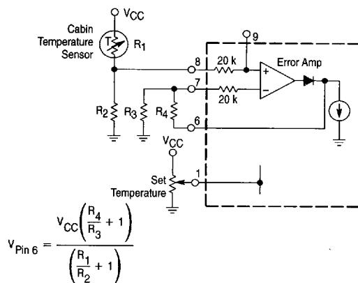
Figure 27. Temperature Sensing Servo System
