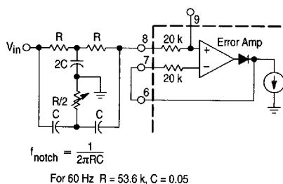
Figure 25. Notch Filter
