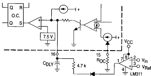
Figure 29. Remote Latched Shutdown
