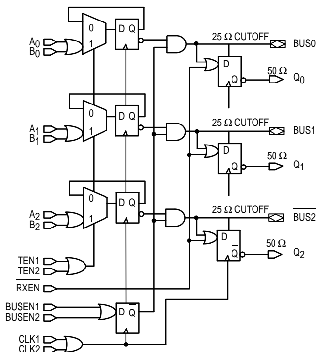
LOGIC DIAGRAM
