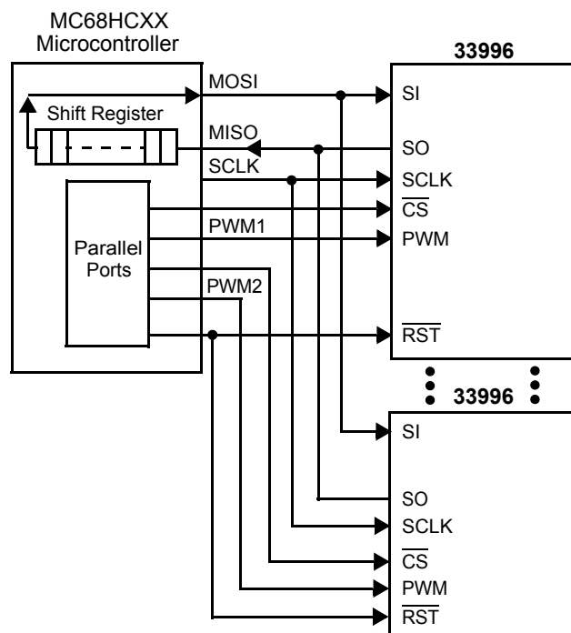
Figure 5. Parallel Inputs SPI Control
