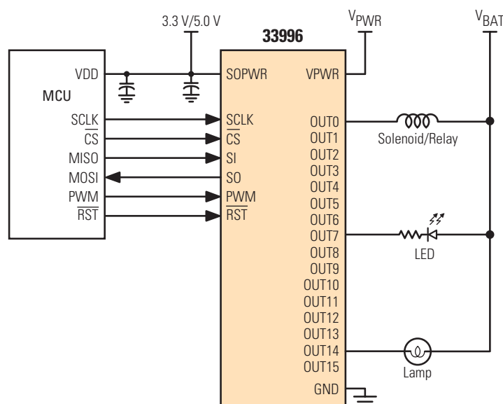
33996 Simplified Application Diagram
