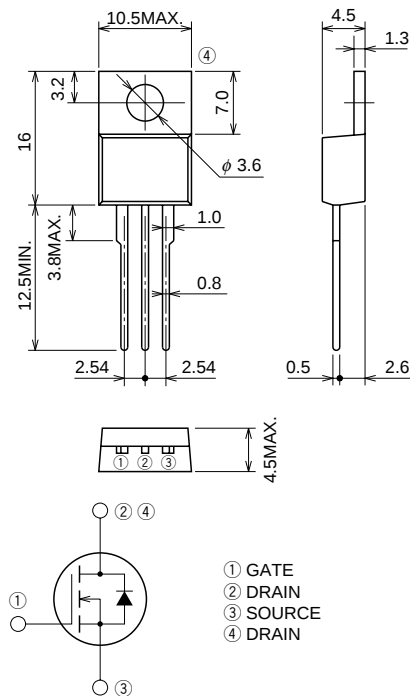
TO-220
