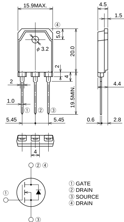
TO-3P
