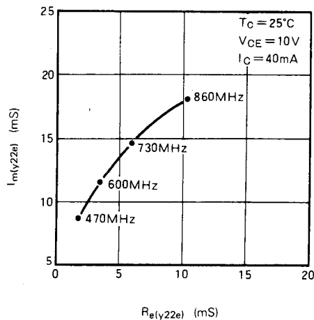
OUTPUT ADMITTANCE VS. FREQUENCY
