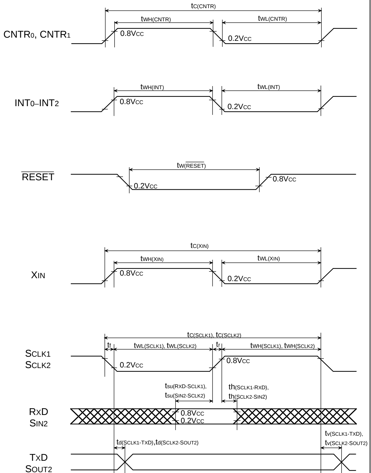
Fig. 57 Timing diagram
