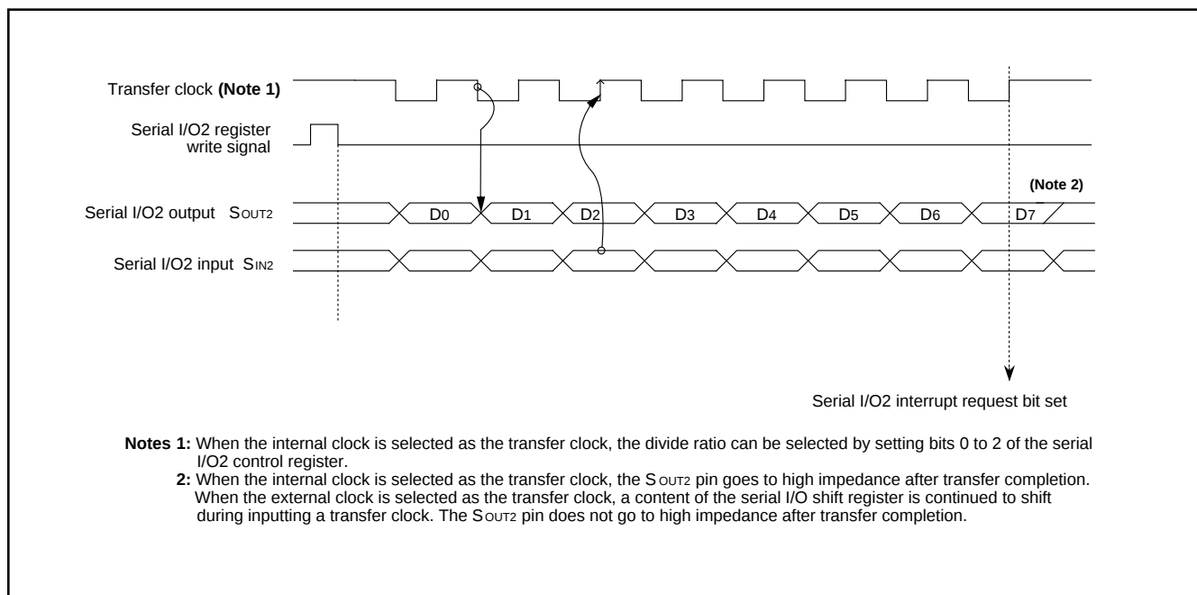
Fig. 30 Timing of serial I/O2 function
