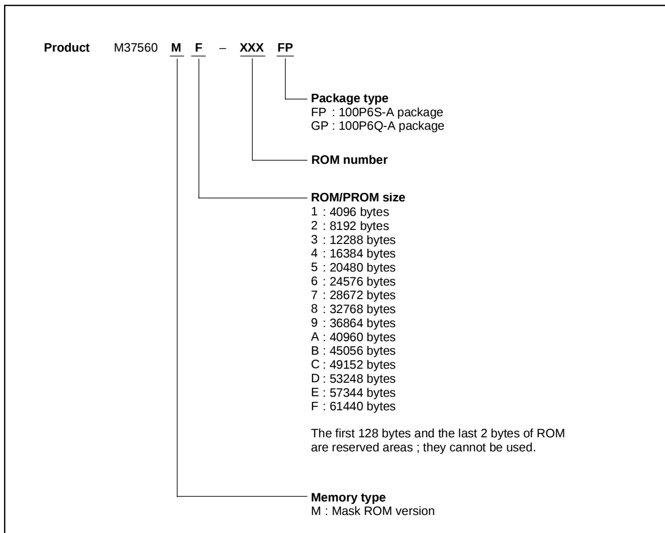
Fig. 4 Part numbering
