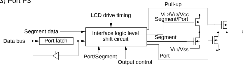
(3) Port P3
