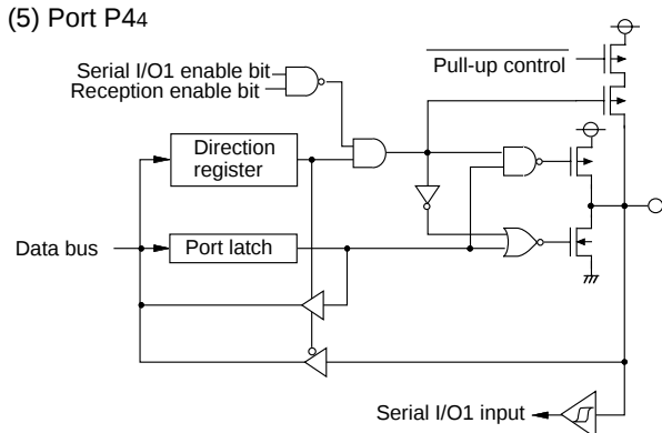
(5) Port P44
