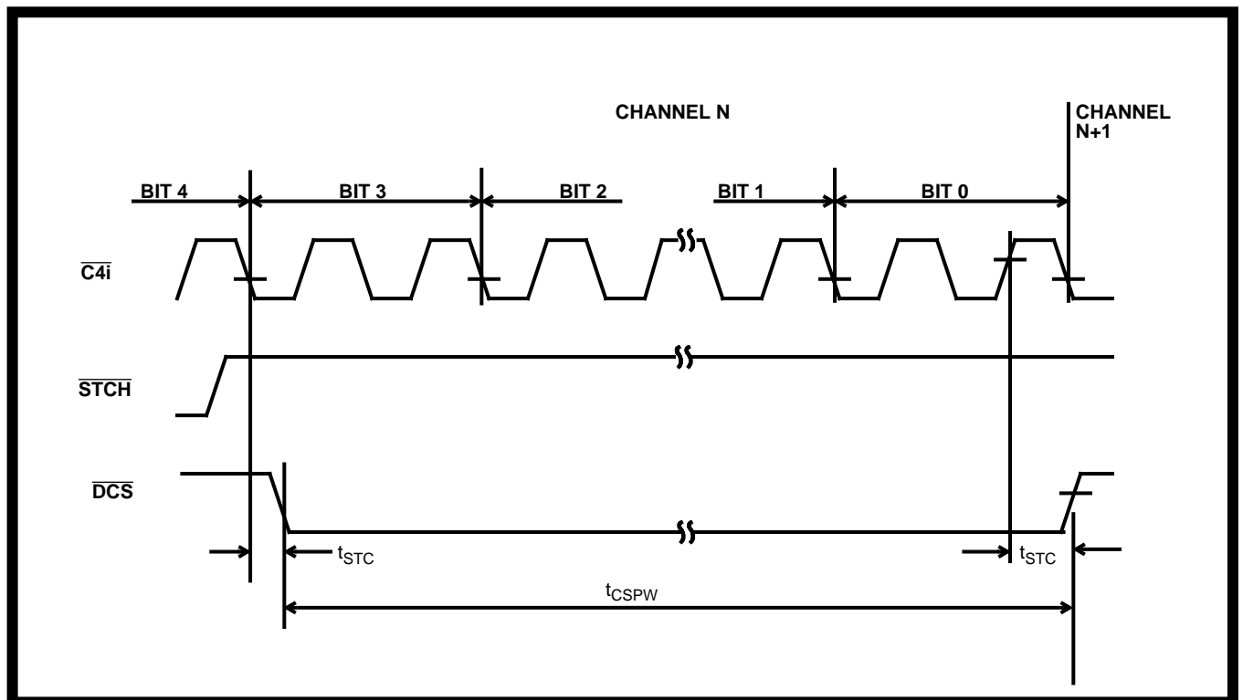
Figure 19 - Mode 3 DCS Timing Diagram
