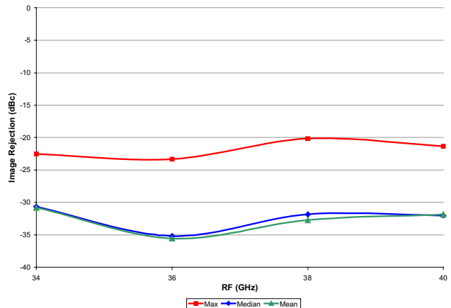
XM1002, USB Image Rejection (6566 devices)
