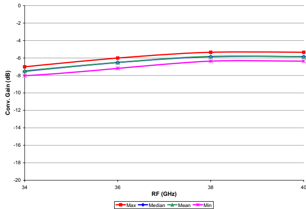
XM1002, USB Conversion Gain (6566 devices)
