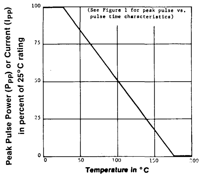
FIGURE 3 Derating Curve
