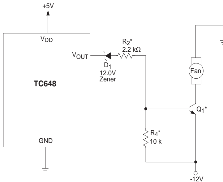
FIGURE 5-7: Powering the Fan from a -12V Supply.
