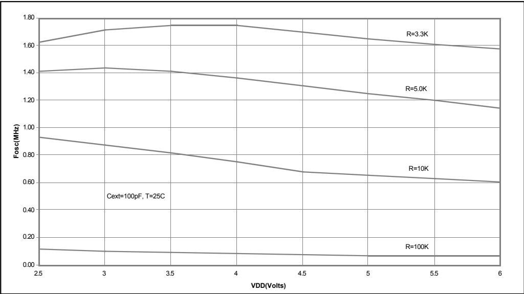
FIGURE 11-3: TYPICAL RC OSCILLATOR FREQUENCY vs. V_{DD} , C_{EXT} = 100\text{ pF}
