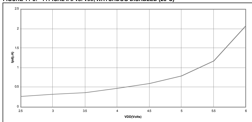
FIGURE 11-5: TYPICAL I_{PD} vs. V_{DD} , WATCHDOG DISABLED ( 25^\circ\text{C} )
