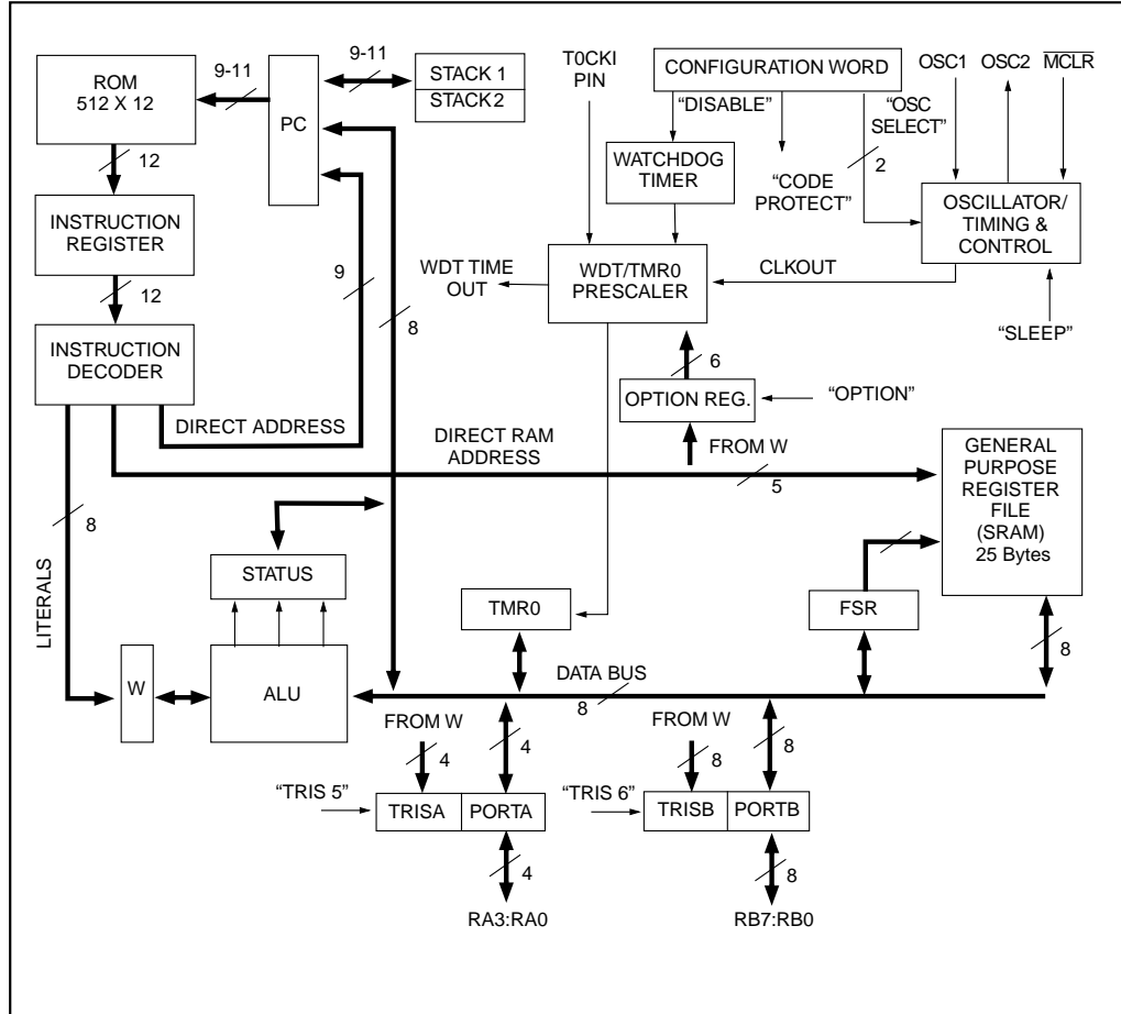
FIGURE 3-1: PIC16CR54C SERIES BLOCK DIAGRAM
