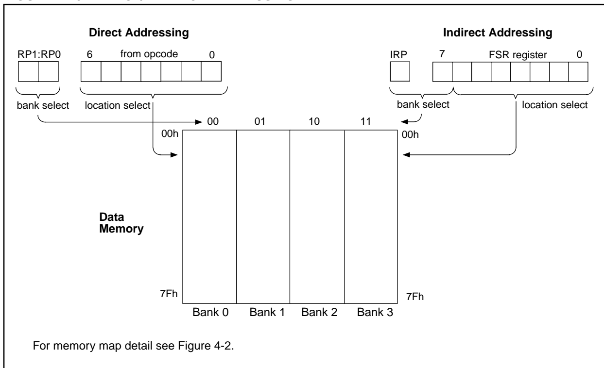
FIGURE 4-10: DIRECT/INDIRECT ADDRESSING
