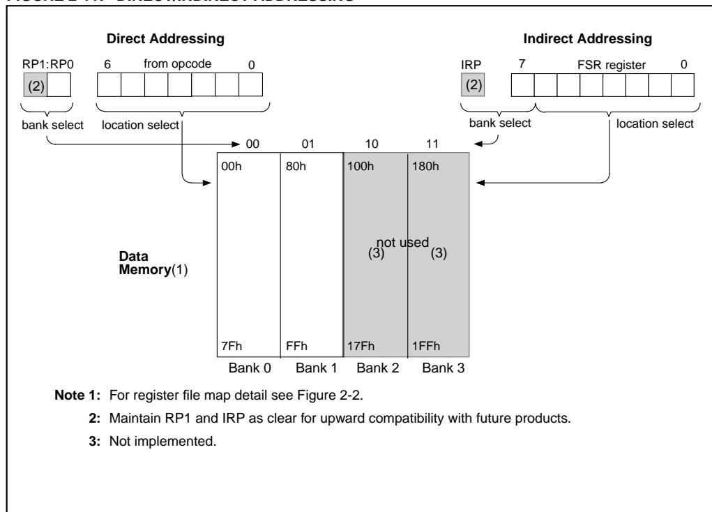
FIGURE 2-11: DIRECT/INDIRECT ADDRESSING
