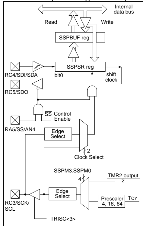
FIGURE 8-6: SSP BLOCK DIAGRAM (SPI MODE)(PIC16C72)
