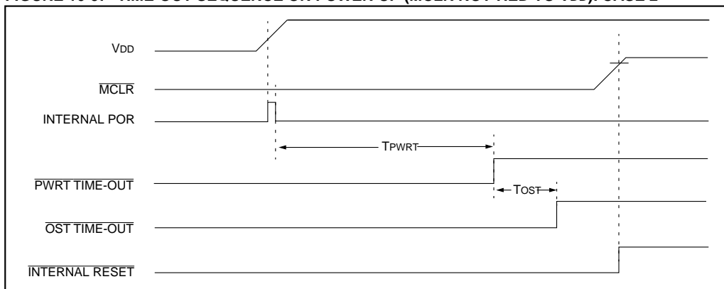
FIGURE 10-9: TIME-OUT SEQUENCE ON POWER-UP (MCLR NOT TIED TO VDD): CASE 2
