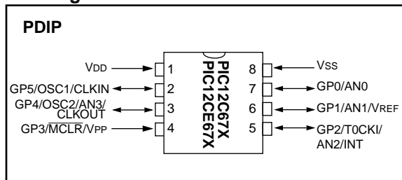
Pin Diagram:
