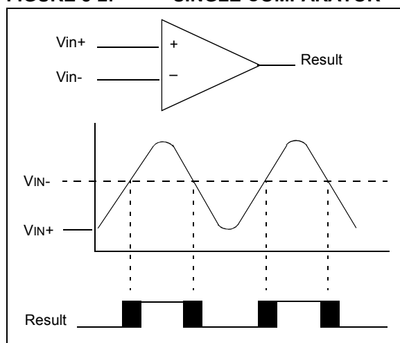
FIGURE 8-2: SINGLE COMPARATOR
