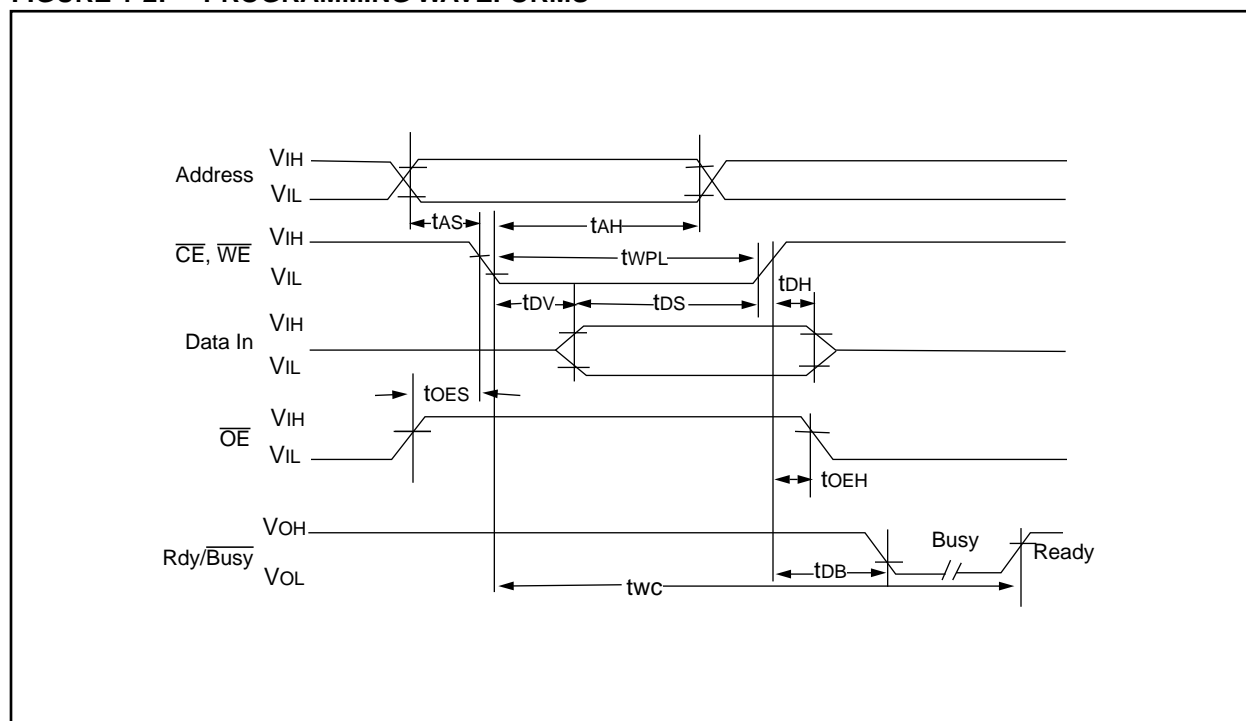
FIGURE 1-2: PROGRAMMING WAVEFORMS
