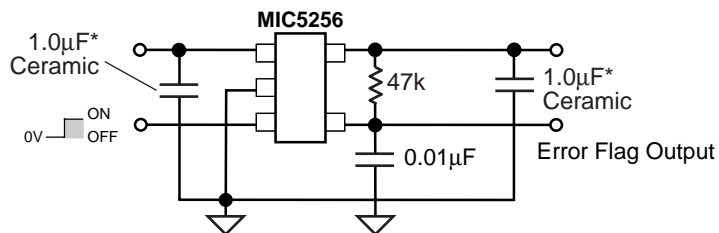
Figure 1. Test Circuit
