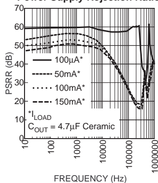
Power Supply Rejection Ratio
