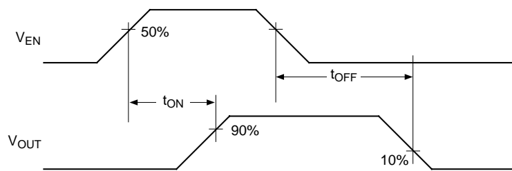
Figure 1a. MIC2546/47-1
