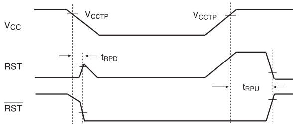
Figure 1. Power-Up/Power-Down Sequence
