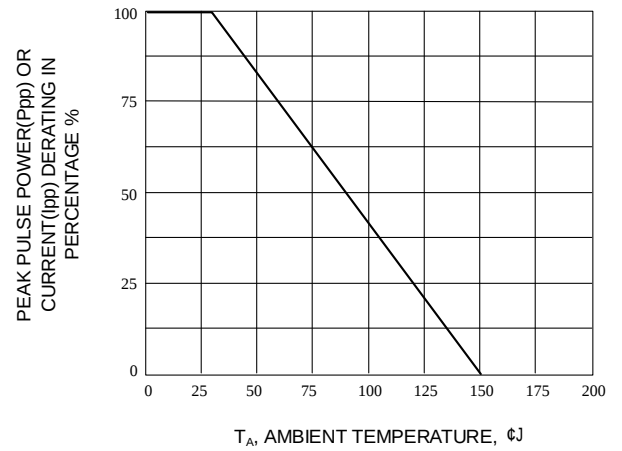
Fig. 2-PULSE RATING CURVE
