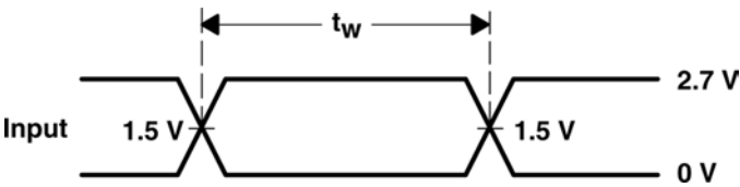
FIGURE 2. PULSE DURATION
