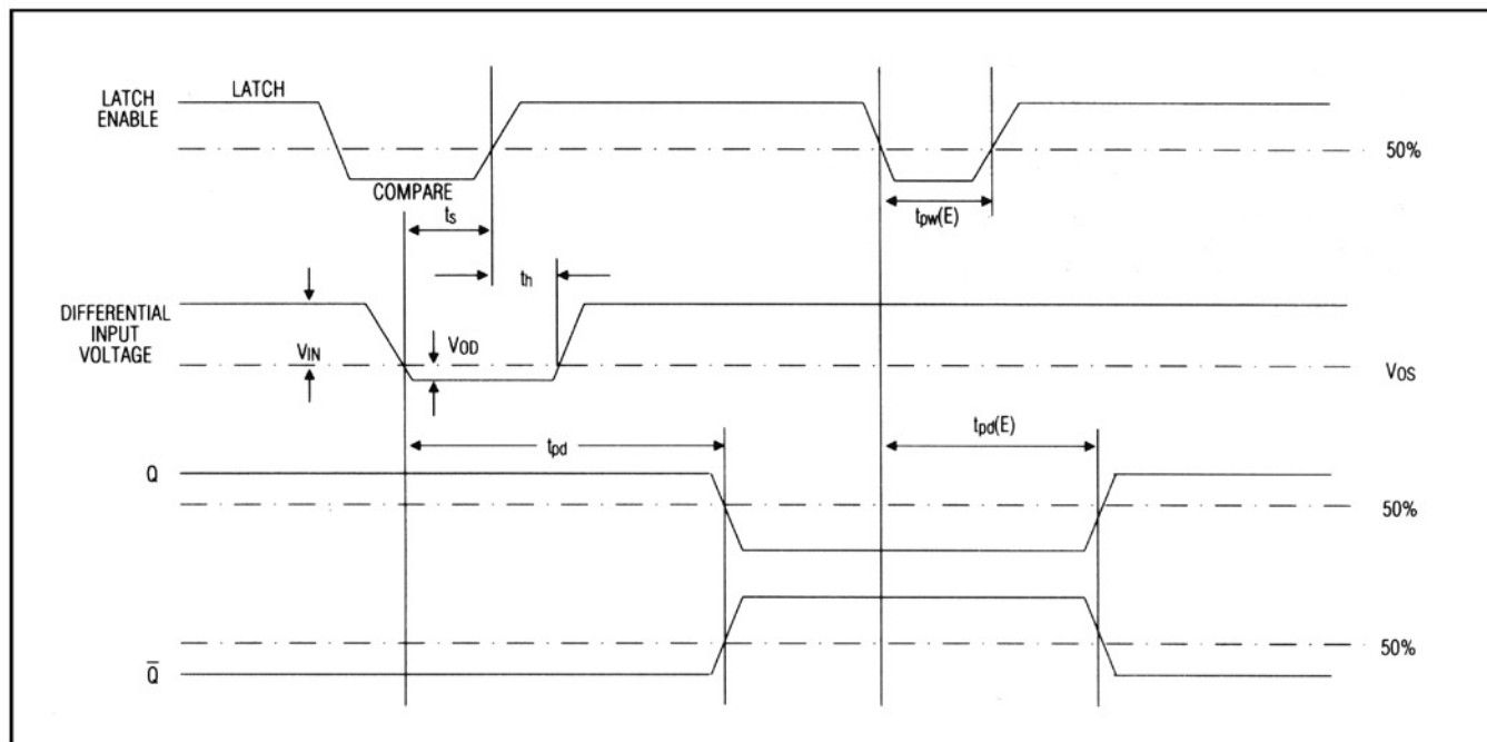
MAX9686 and MAX9698 Timing Diagram (worst case)
