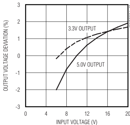
OUTPUT VOLTAGE DEVIATION vs. INPUT VOLTAGE
