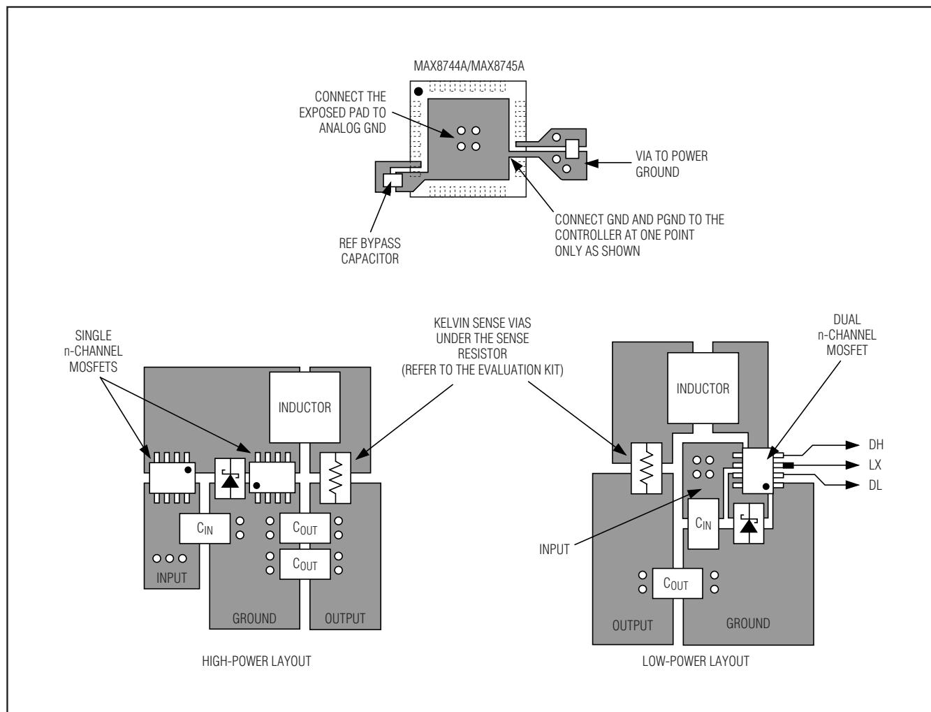
Figure 9. PCB Layout
