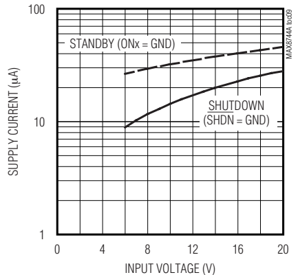
STANDBY AND SHUTDOWN INPUT CURRENT vs. INPUT VOLTAGE
