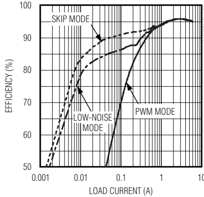
3.3V OUTPUT EFFICIENCY vs. LOAD CURRENT
