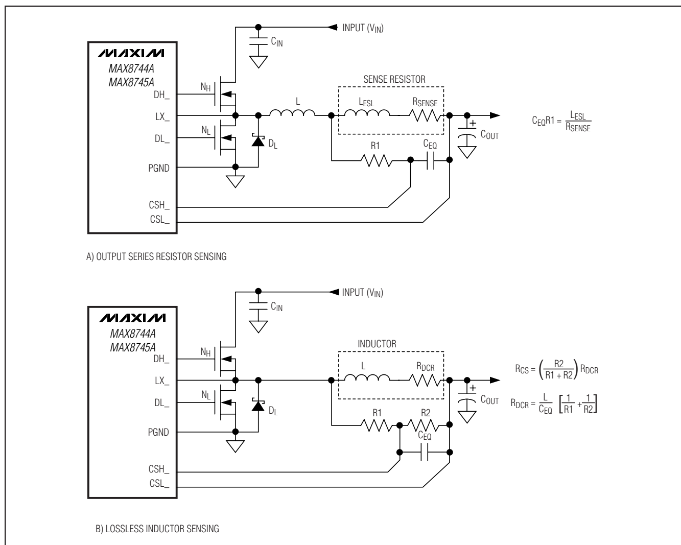
Figure 7. Current-Sense Configurations
