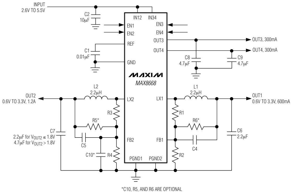
Figure 4. MAX8668 Typical Application Circuit
